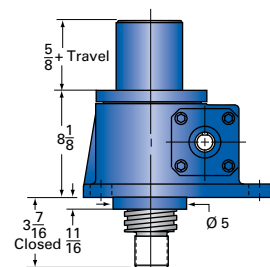
30-MSJ-I INVERTED
