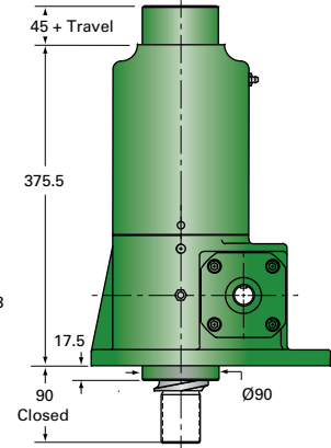
EM20-BSJ-I INVERTED
