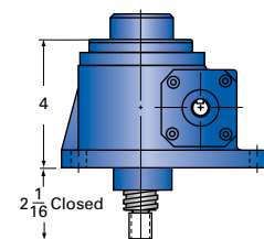
2.5AB-MSJ-I INVERTED ANTI-BACKLASH
