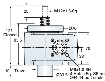
EM1-MSJ-U UPRIGHT
