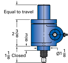
MJ-xx-I INVERTED
