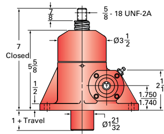
2R-BSJ-U UPRIGHT
